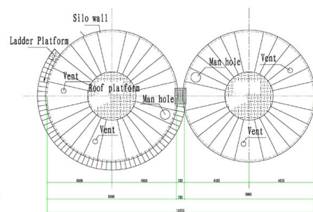
ø8 Silo Layout
